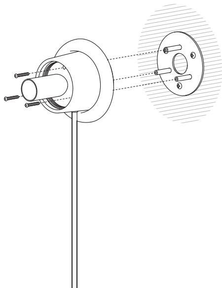
Step 4. Securing Body to Bracket
