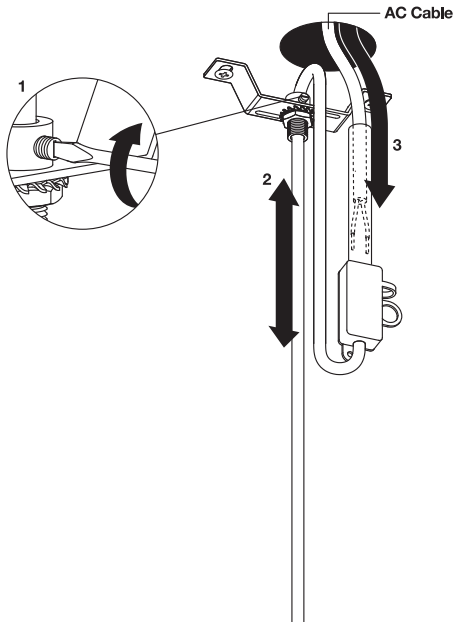
Step 3. Adjusting the Cable Length
