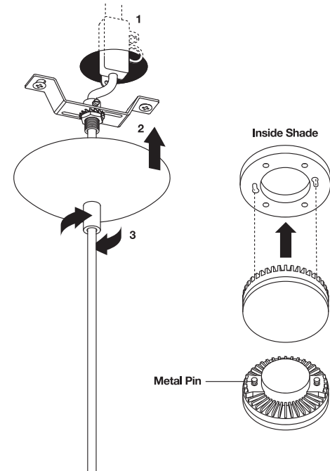
Step 6. Securing Ceiling Cover and Assembling the Bulb
