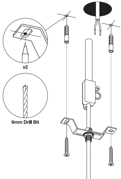
Step 2. Installing Bracket on the Ceiling
