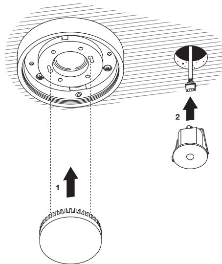
Step 6. Assembling the LED Bulb and Sensor
