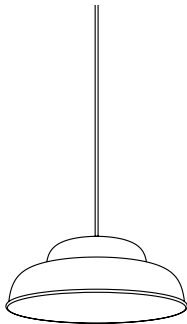
FROG40 Pendant White, Butter, Deep Green AL + Steel + Zinc 400 x 400 x 158mm / 1.55kg LED GX53 FLAT 8W 2700K, 4000K AC 220V
