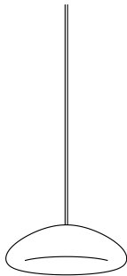
BELLY30 Pendant White, Sand, Terracotta AL + Steel 300 x 300 x 100mm / 1.55kg LED GX53 FLAT 8W 2700K, 4000K AC 220V
