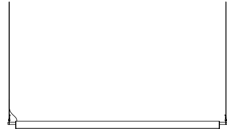
PINOCCHIO120 Pendant White, Silver, Black Body : Aluminum + PC Cable A : Stainless Steel Cable B, C : Polyester 1200 x 35 x 40mm 1.65kg Flicker Free Integrated LED 25W 3000K AC 220V
