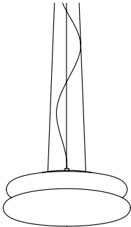
SNOWMAN40 Pendant AL + Glass 400 x 400 x 160mm 2.6kg AC 220V Integrated LED 15W 3000K
